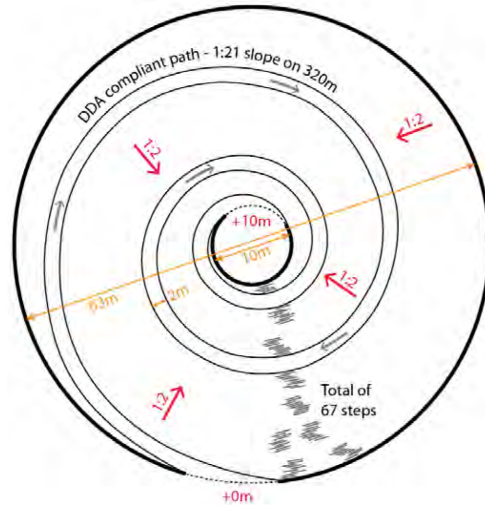
Diagrammatic plan view
